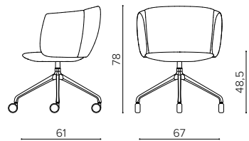
NT 5098R SMALL 4-spoke aluminum swivel base on casters base girevole a 4 razze in alluminio su ruote
