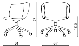
NT 509C SMALL 5-spoke aluminum swivel base on casters base girevole a 5 razze in alluminio su ruote
